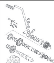
Kickstarter
